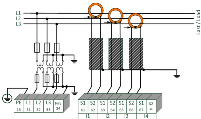
Example of PQI-DA smart connection with Rogowski coils in a 3-wire network
