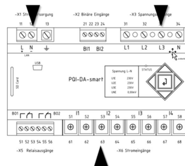
Position of the mounting elements
