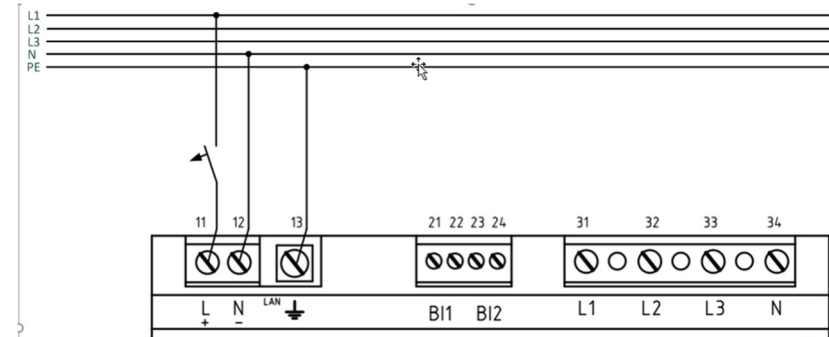
Example of connection to 230V AC with feature
