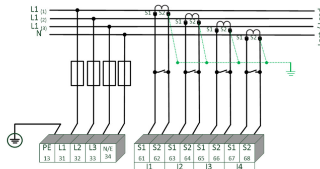
PQI-DA smart in 4-wire connection -1-phase
