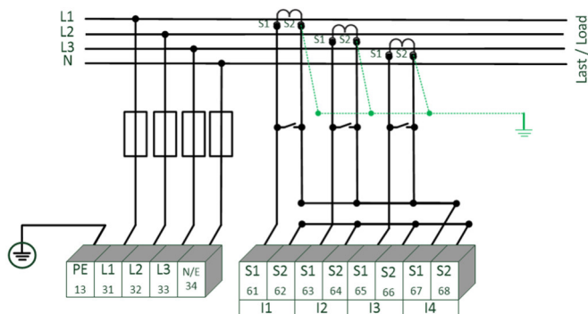
PQI-DA smart without neutral conductor of current transformer in 4-wire connection
